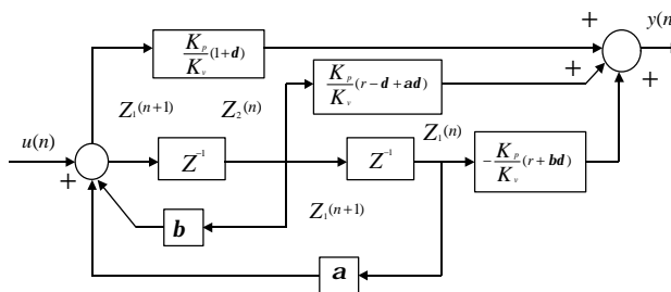
Figure 4. Discrete model of AC servo motor.
