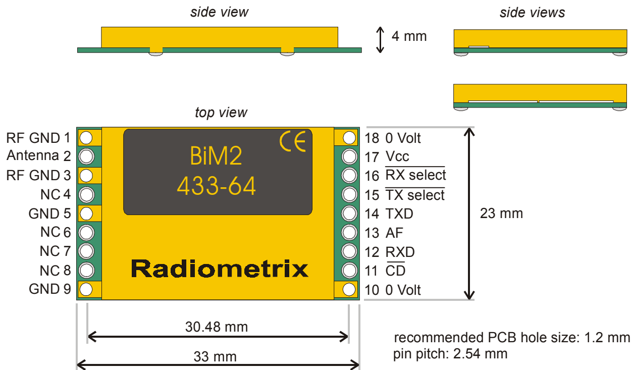
Figure 2: Physical dimension
